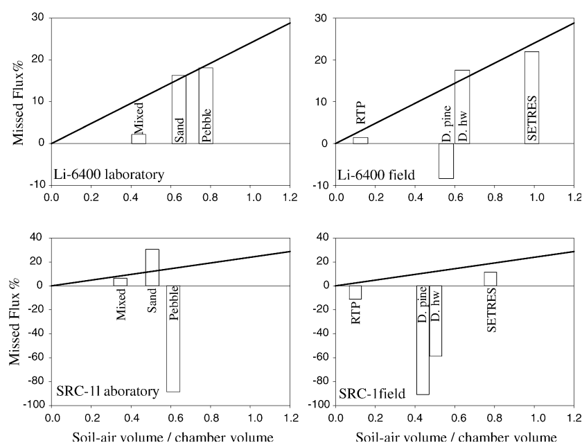
Figure 3. Comparison of flux underestimation (missed flux) by closed chamber techniques with the ratio of soil–air volume and measurement chamber volume. Missed flux is the % underestimation relative to the generated flux 1 - (\text{observed/expected}) \times 100 . Soil–air volume was directly measured in the laboratory apparatus for each soil medium. For the field results, air-filled porosity was measured at the time of respiration sampling and an assumed soil depth of 30 cm was used to calculate soil volume for comparison. In the field experiment there is no definitive value of missed flux. The solid line represents the relationship predicted by Conen and Smith (2000).
