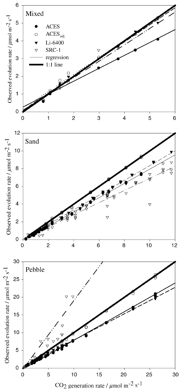
Figure 1. Comparison of CO 2 flux generated through three artificial soil media, and measurements made with the ACES (raw data and adj), the Li-6400-09 and the SRC-1. The solid line represents a 1:1 ratio and the expected value. Linear regression equations and R^2 values are presented in Table 2.
