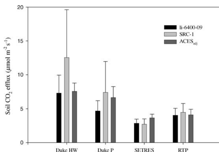
Figure 2. Mean soil CO 2 flux ( n = 15 , \pm s.d.) measured at four field sites in central North Carolina.
